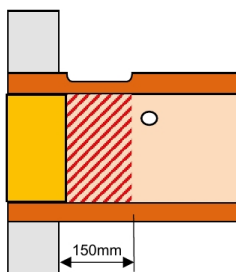
Masonry support
