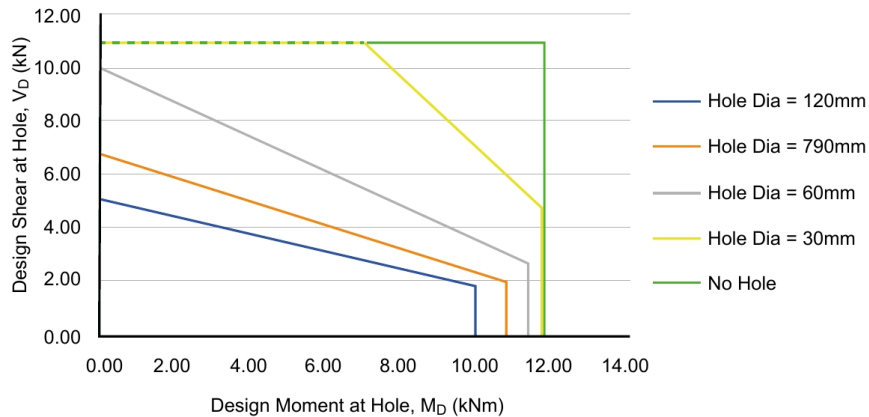
Circular Hole Chart 47 x 300 GL24 Beam
